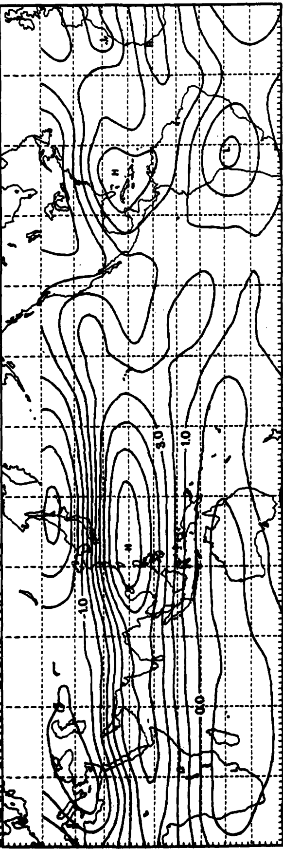
STREAM FUNCTION 200MB WIN 1975
